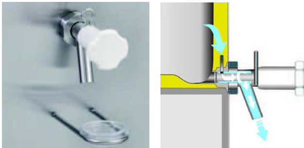
Outlet spigot with independent washing system
