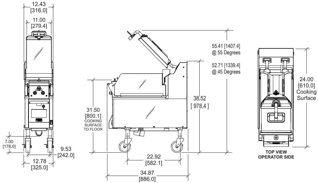
FIGURES IN BRACKETS INDICATE MILLIMETERS / DECIMAL AND FRACTIONAL DIMENSIONS EQUAL TO ( PLUS OR MINUS 1/16 INCH [1.5mm] ). MACHINE HEIGHT CAN VARY ( PLUS OR MINUS 3 INCHES [76.2MM] ) WITH CASTER HEIGHT ADJUSTMENT
